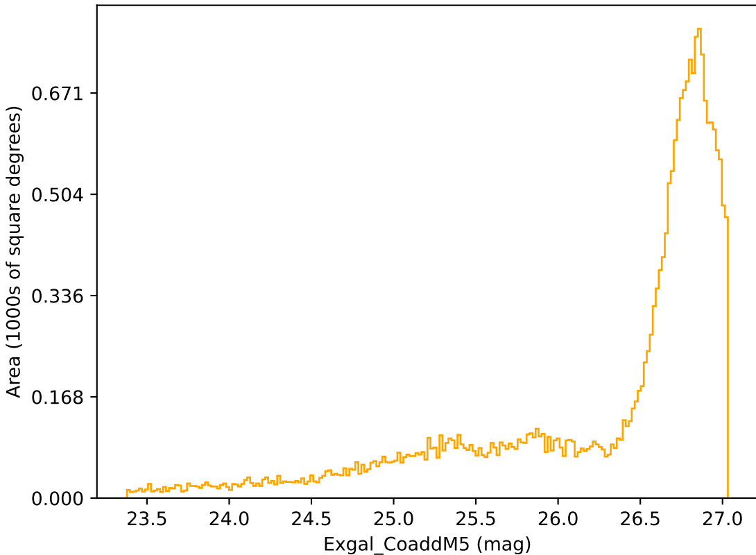
scp_reweight_v3.3_10yrs All sky r band: Exgal_CoaddM5
