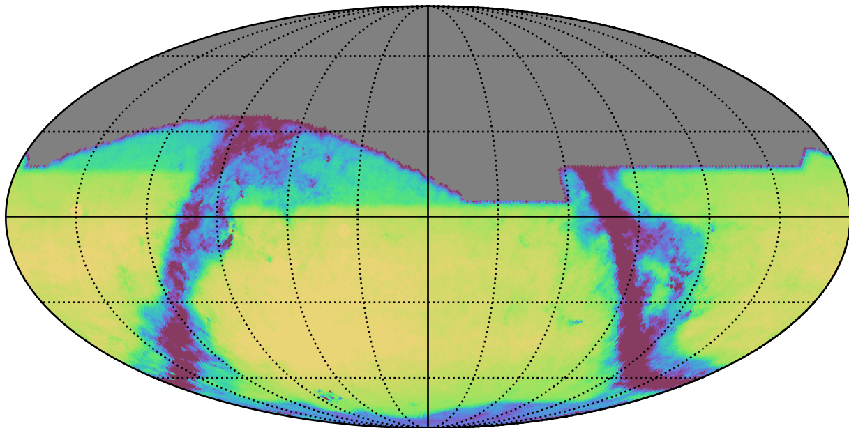
scp_reweight_v3.3_10yrs All sky i band: Exgal_CoaddM5
