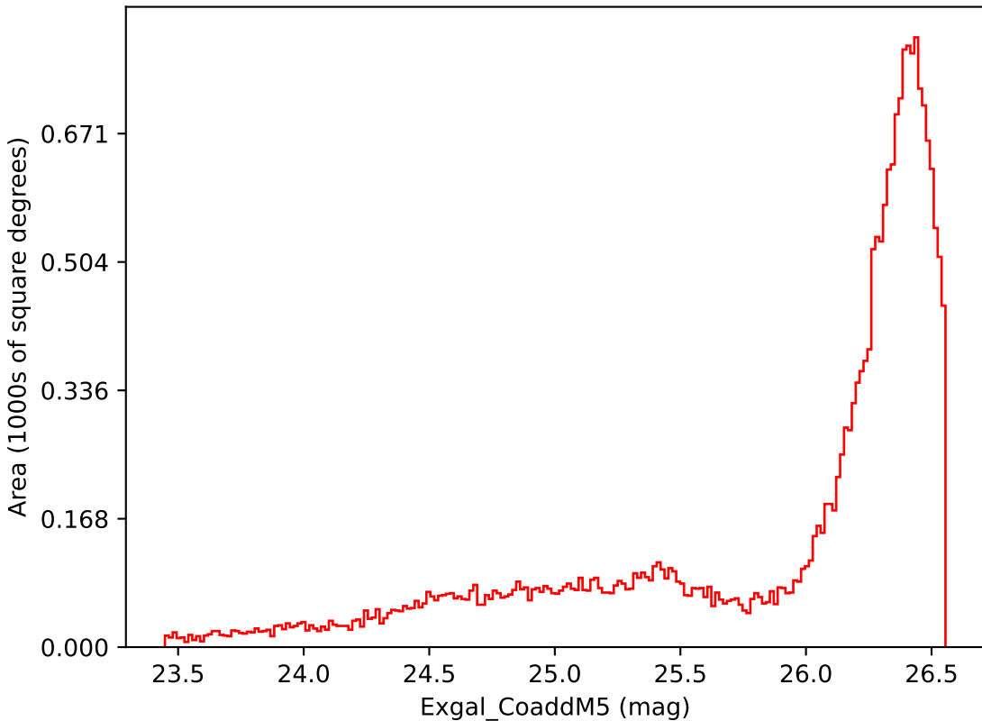
scp_reweight_v3.3_10yrs All sky i band: Exgal_CoaddM5
