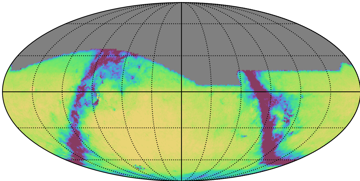
scp_reweight_v3.3_10yrs All sky g band: Exgal_CoaddM5
