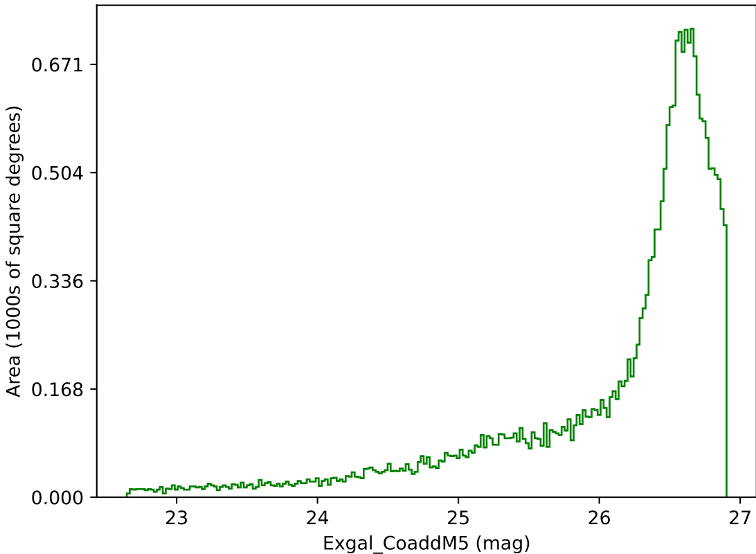
scp_reweight_v3.3_10yrs All sky g band: Exgal_CoaddM5
