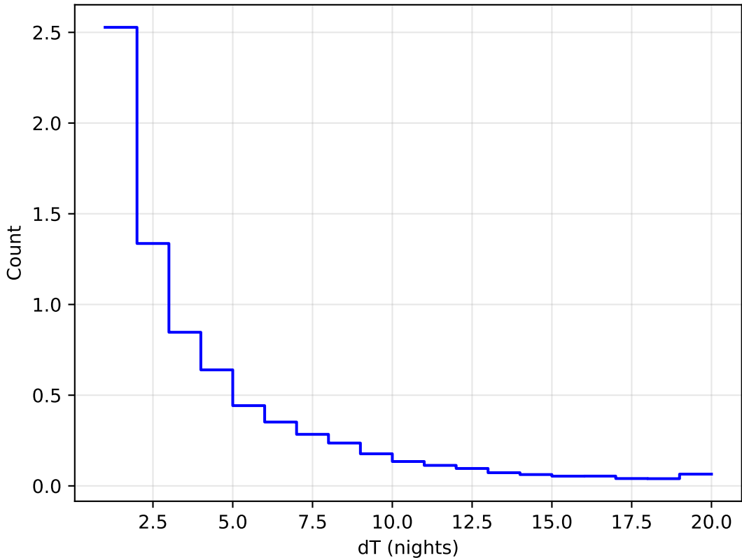
scp_reweight_v3.3_10yrs WFD all bands: DeltaNight Histogram 1e6
