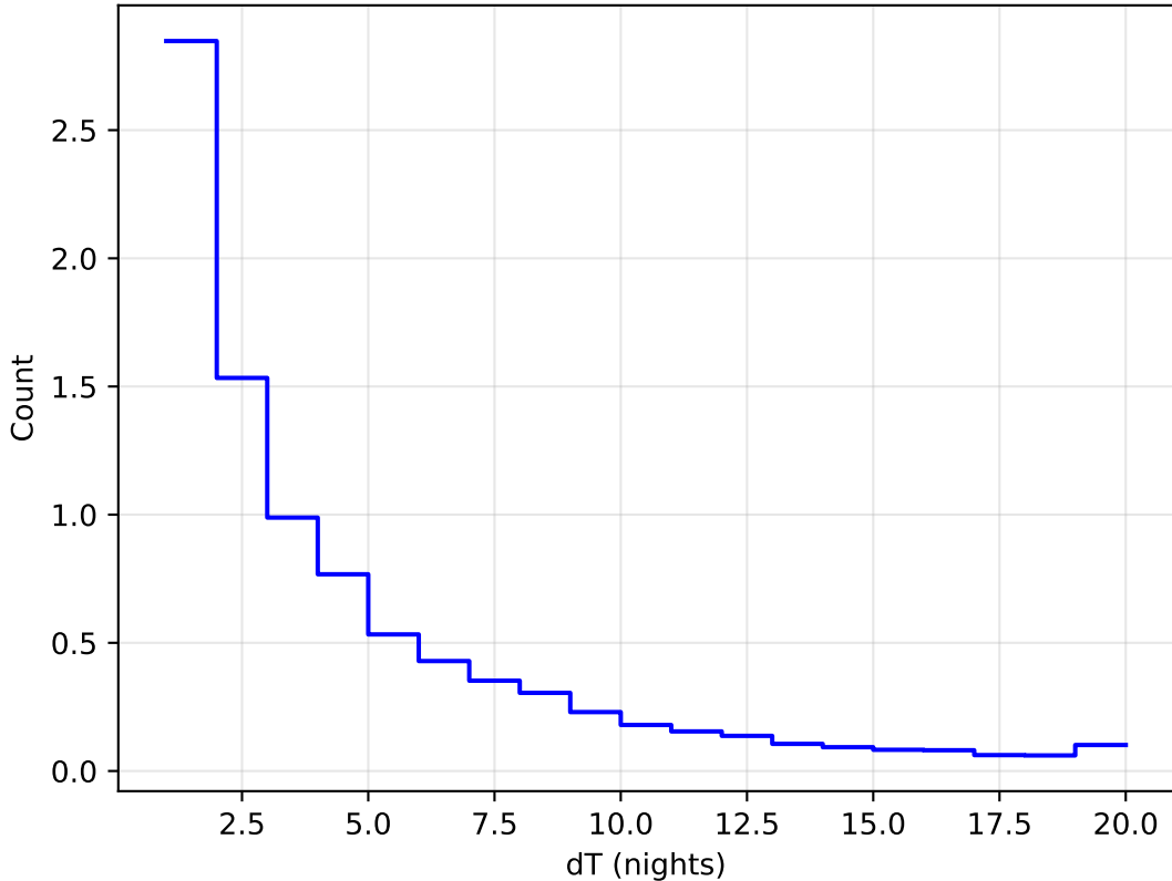
scp_reweight_v3.3_10yrs All sky all bands: DeltaNight Histogram
