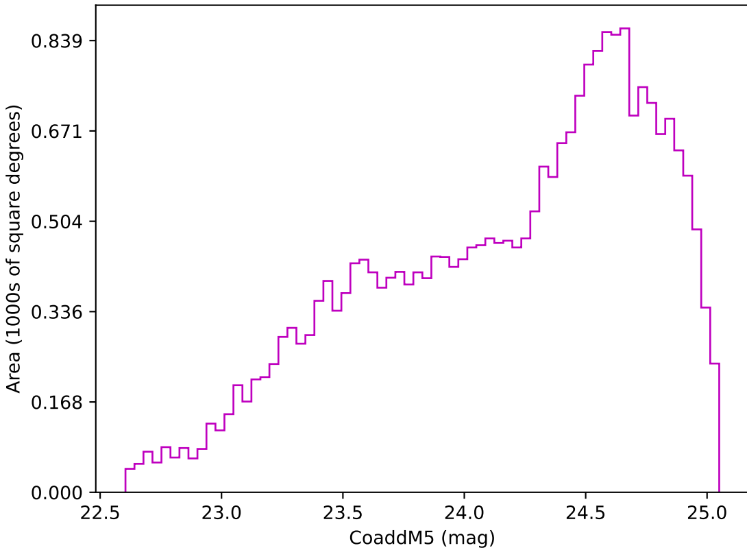
scp_reweight_v3.3_10yrs Yr 3-4 z band: CoaddM5
