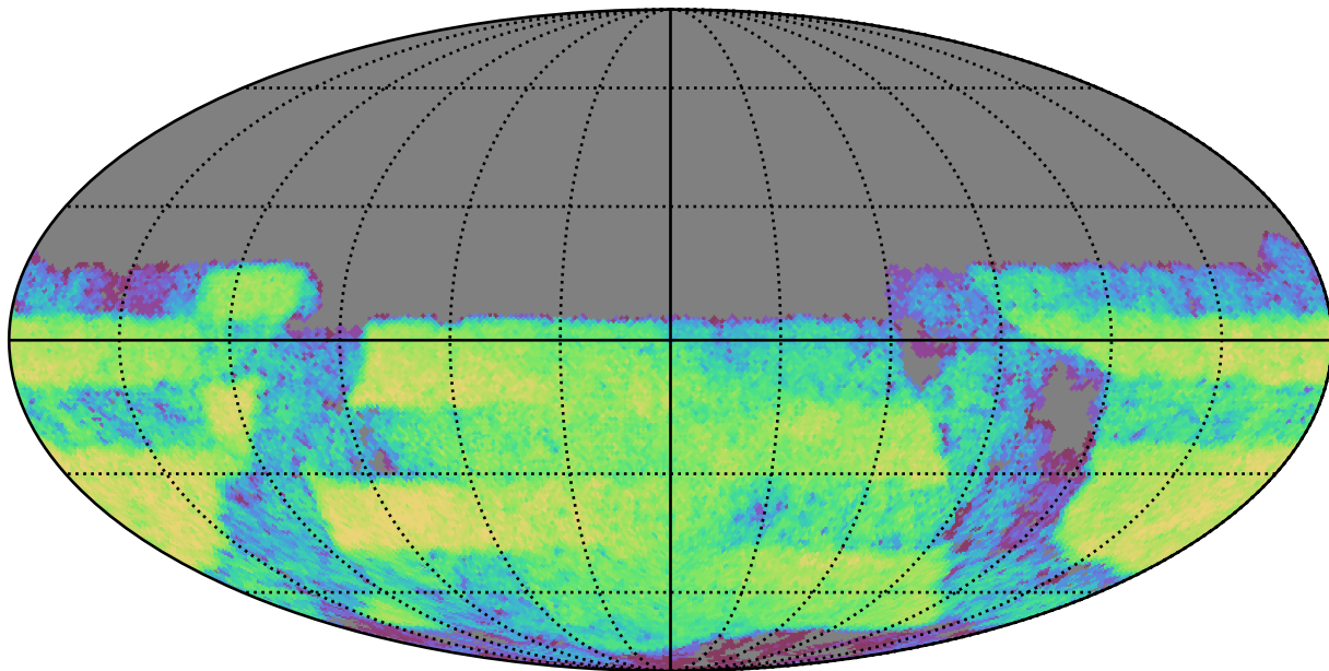
scp_reweight_v3.3_10yrs Yr 3-4 y band: CoaddM5
