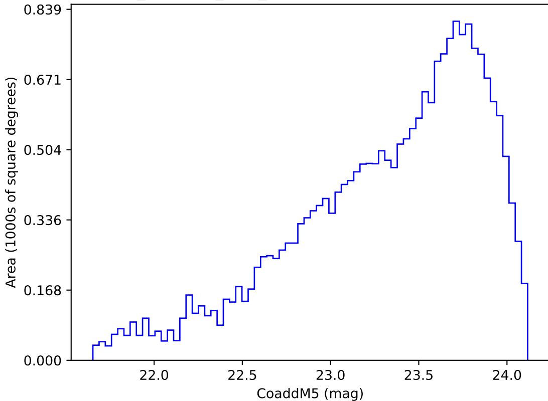
scp_reweight_v3.3_10yrs Yr 3-4 y band: CoaddM5
