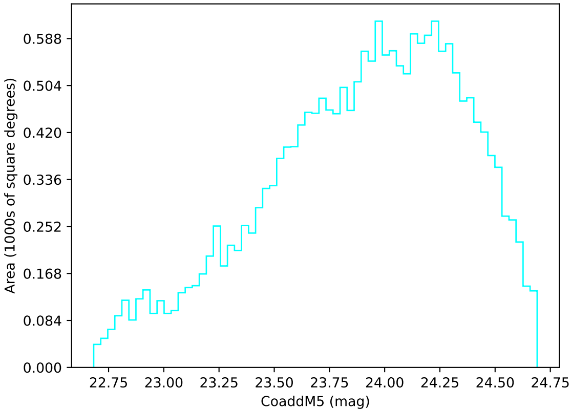
scp_reweight_v3.3_10yrs Yr 3-4 u band: CoaddM5
