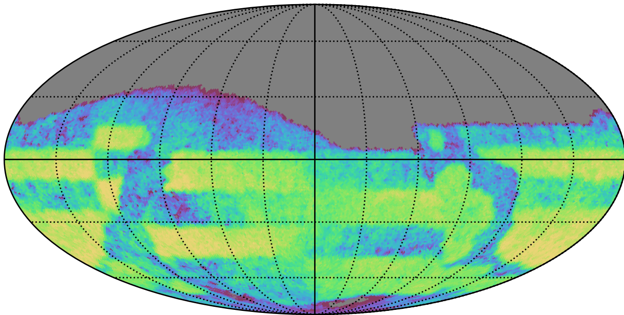
scp_reweight_v3.3_10yrs Yr 3-4 r band: CoaddM5
