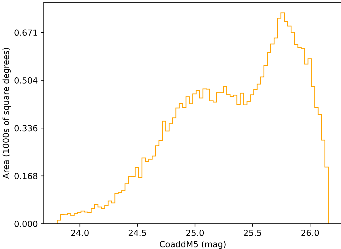
scp_reweight_v3.3_10yrs Yr 3-4 r band: CoaddM5
