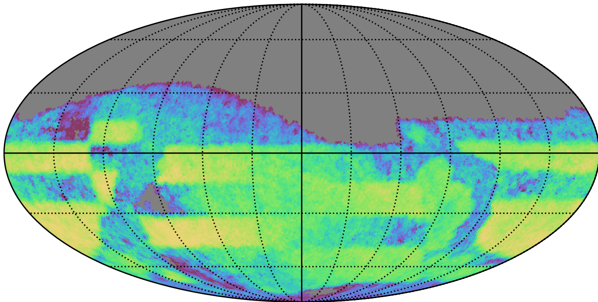
scp_reweight_v3.3_10yrs Yr 3-4 i band: CoaddM5
