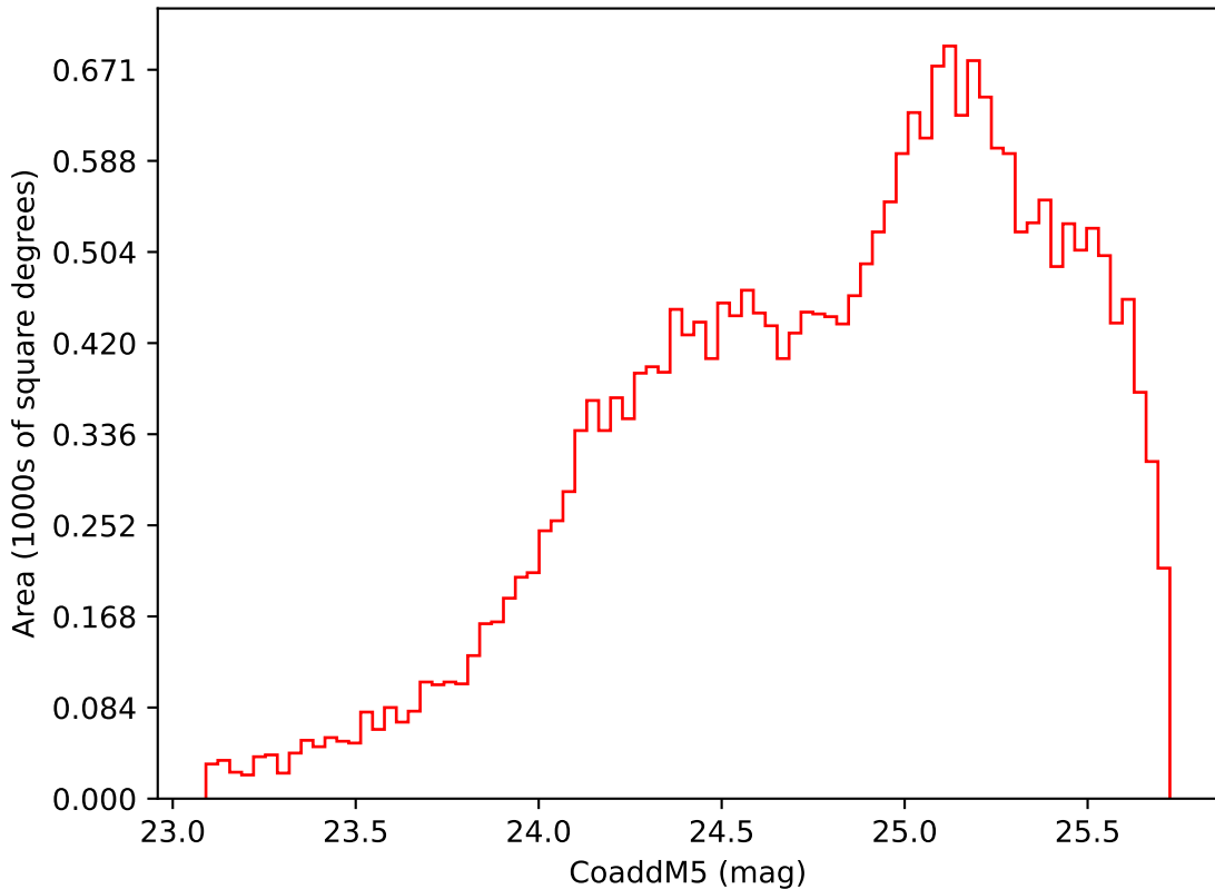
scp_reweight_v3.3_10yrs Yr 3-4 i band: CoaddM5
