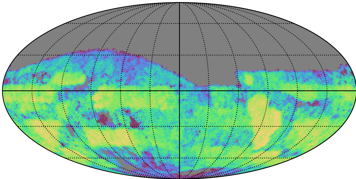
scp_reweight_v3.3_10yrs Yr 3-4 g band: CoaddM5
