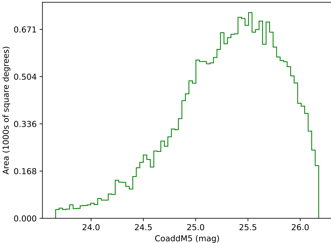
scp_reweight_v3.3_10yrs Yr 3-4 g band: CoaddM5
