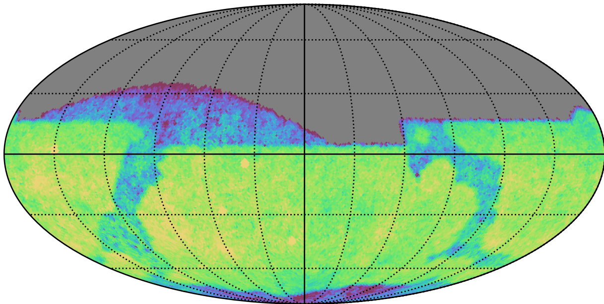
scp_reweight_v3.3_10yrs Yr 1 z band: CoaddM5
