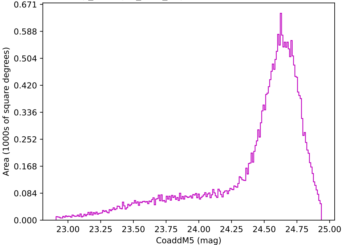
scp_reweight_v3.3_10yrs Yr 1 z band: CoaddM5
