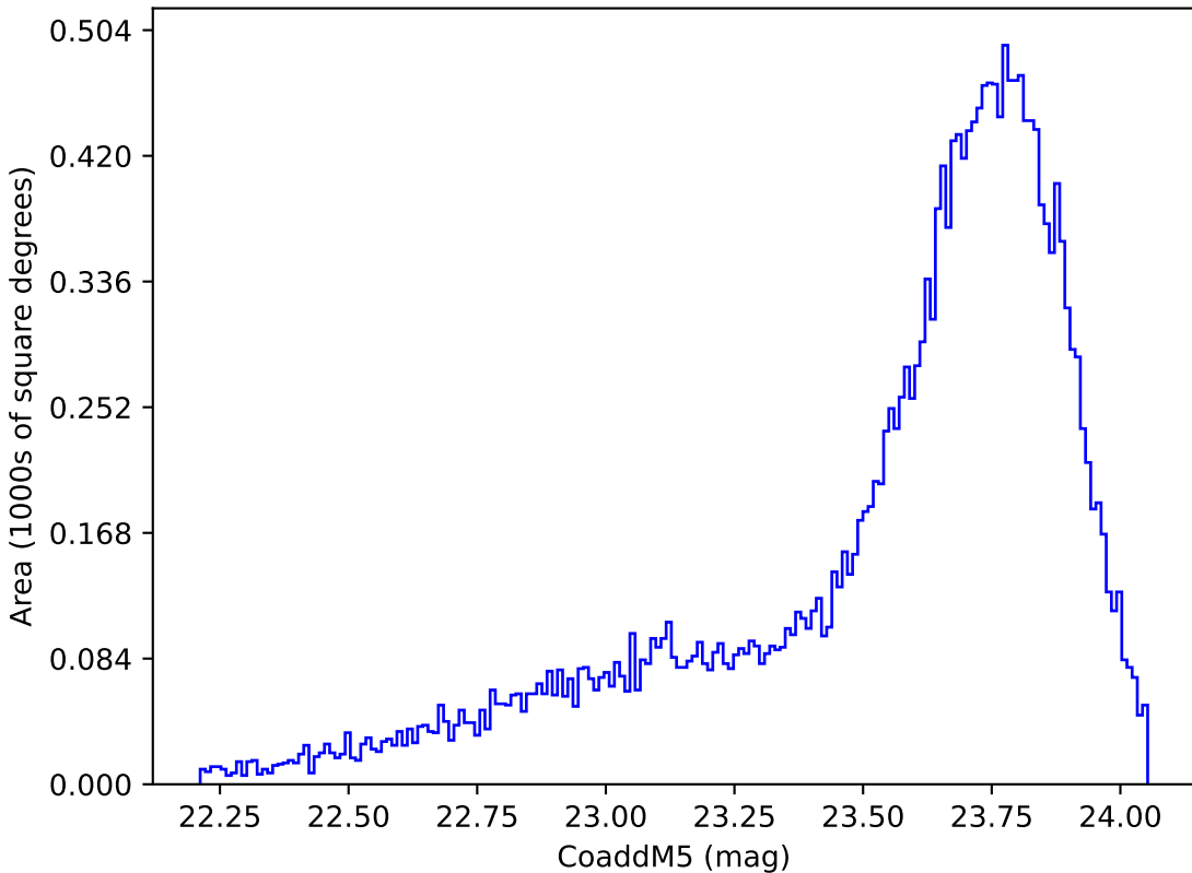
scp_reweight_v3.3_10yrs Yr 1 y band: CoaddM5
