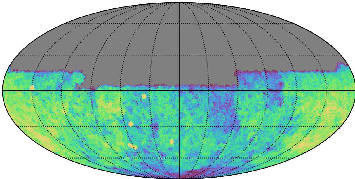
scp_reweight_v3.3_10yrs Yr 1 u band: CoaddM5
