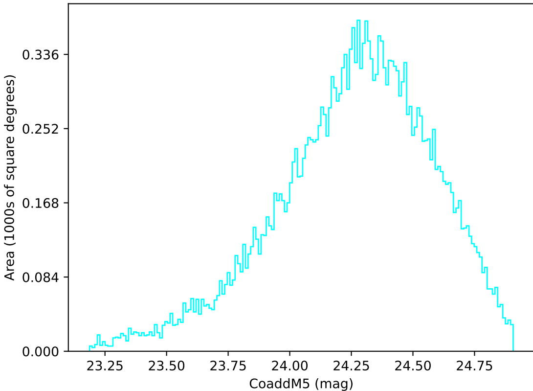
scp_reweight_v3.3_10yrs Yr 1 u band: CoaddM5
