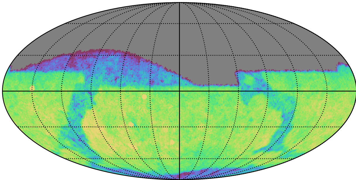
scp_reweight_v3.3_10yrs Yr 1 r band: CoaddM5
