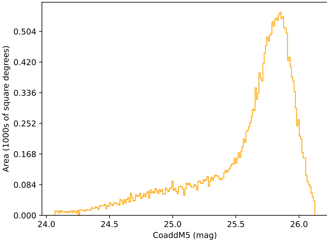
scp_reweight_v3.3_10yrs Yr 1 r band: CoaddM5
