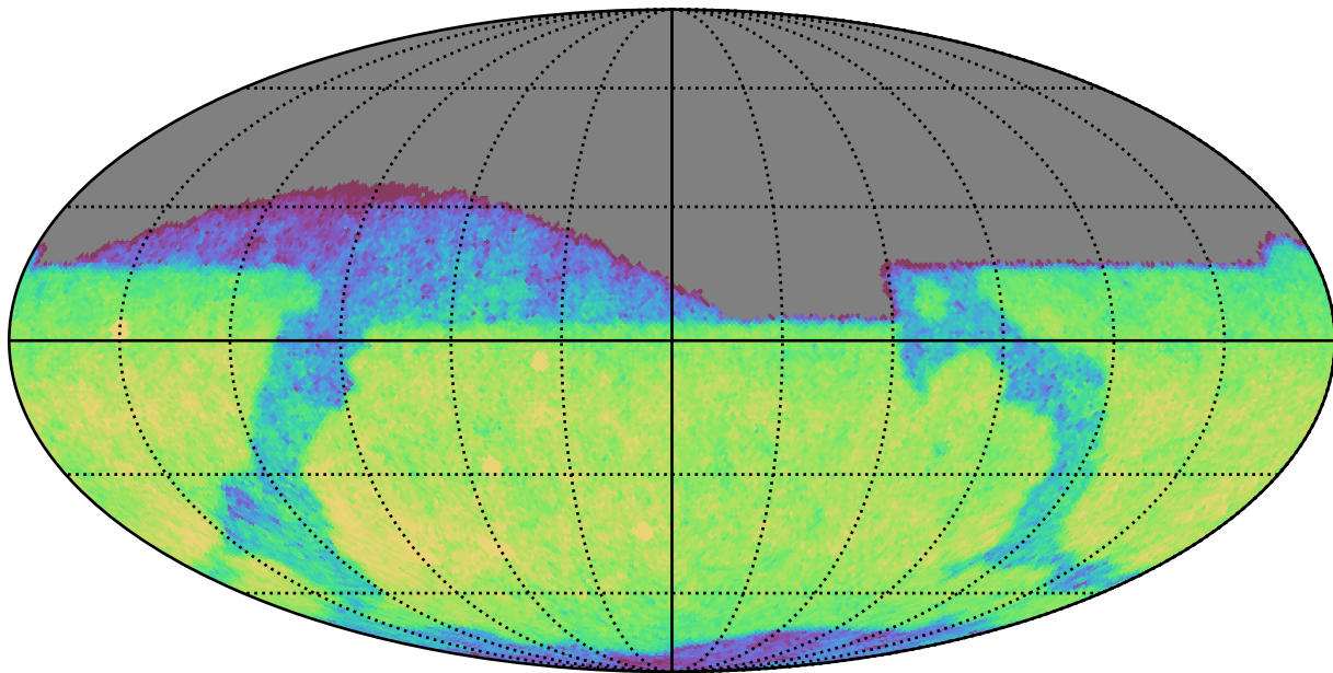
scp_reweight_v3.3_10yrs Yr 1 i band: CoaddM5
