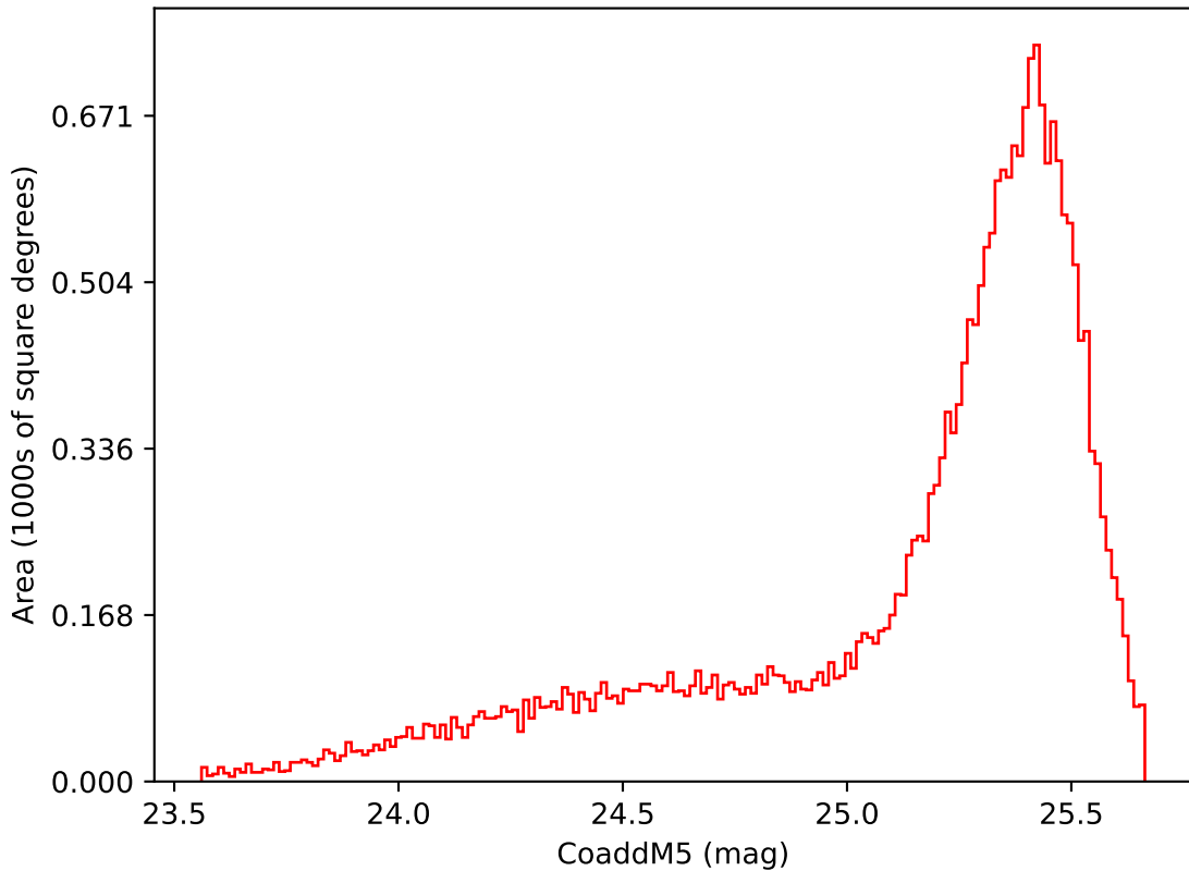
scp_reweight_v3.3_10yrs Yr 1 i band: CoaddM5
