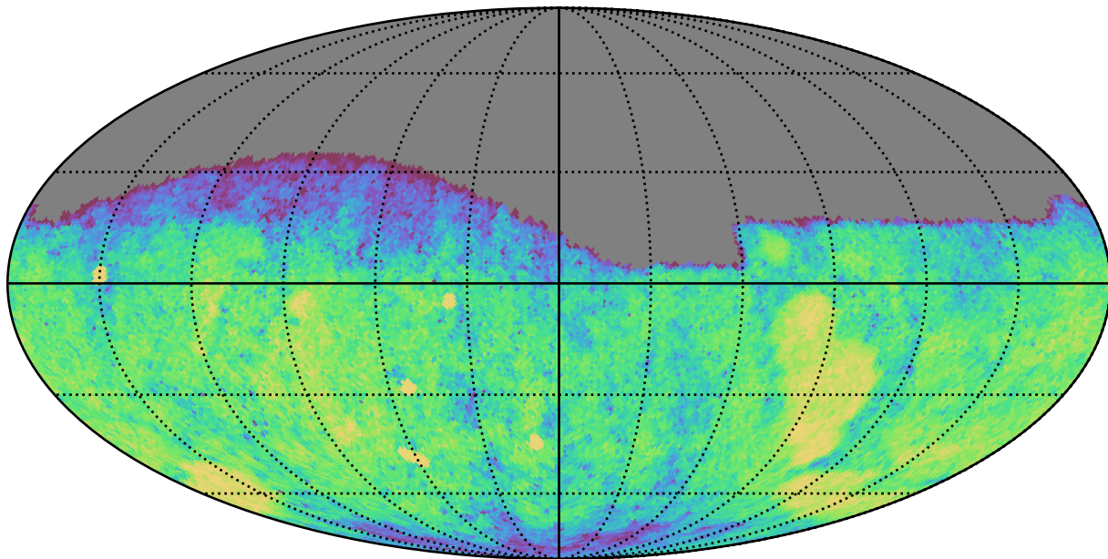
scp_reweight_v3.3_10yrs Yr 1 g band: CoaddM5
