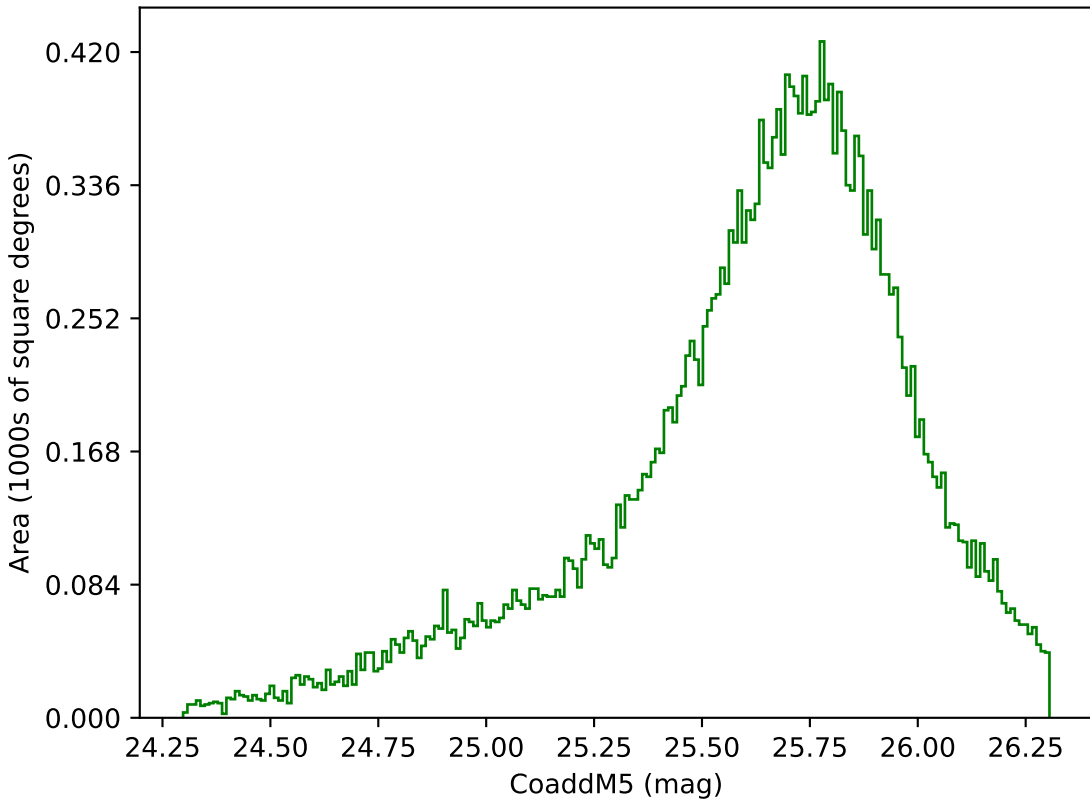
scp_reweight_v3.3_10yrs Yr 1 g band: CoaddM5
