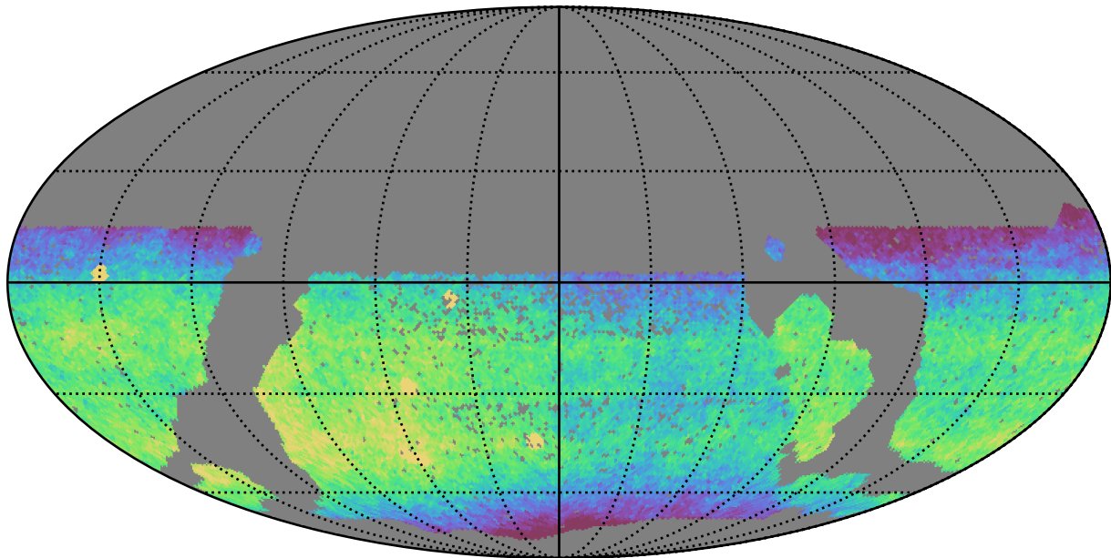
scp_reweight_v3.3_10yrs WFD z band: CoaddM5
