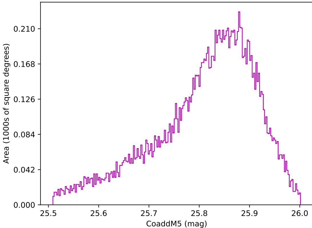
scp_reweight_v3.3_10yrs WFD z band: CoaddM5
