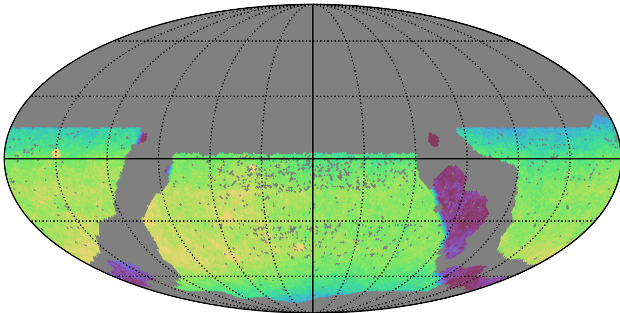
scp_reweight_v3.3_10yrs WFD y band: CoaddM5
