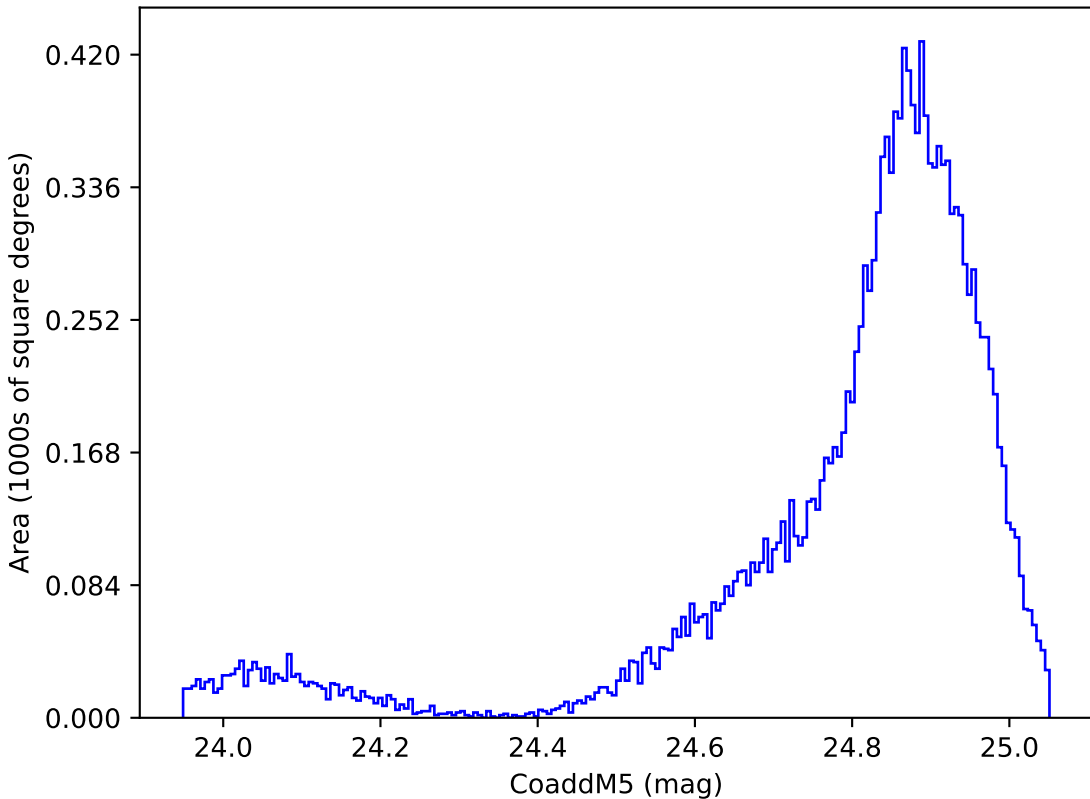
scp_reweight_v3.3_10yrs WFD y band: CoaddM5
