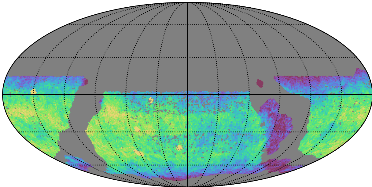
scp_reweight_v3.3_10yrs WFD u band: CoaddM5
