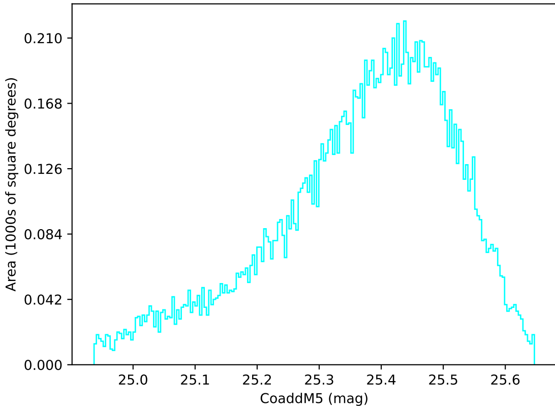
scp_reweight_v3.3_10yrs WFD u band: CoaddM5
