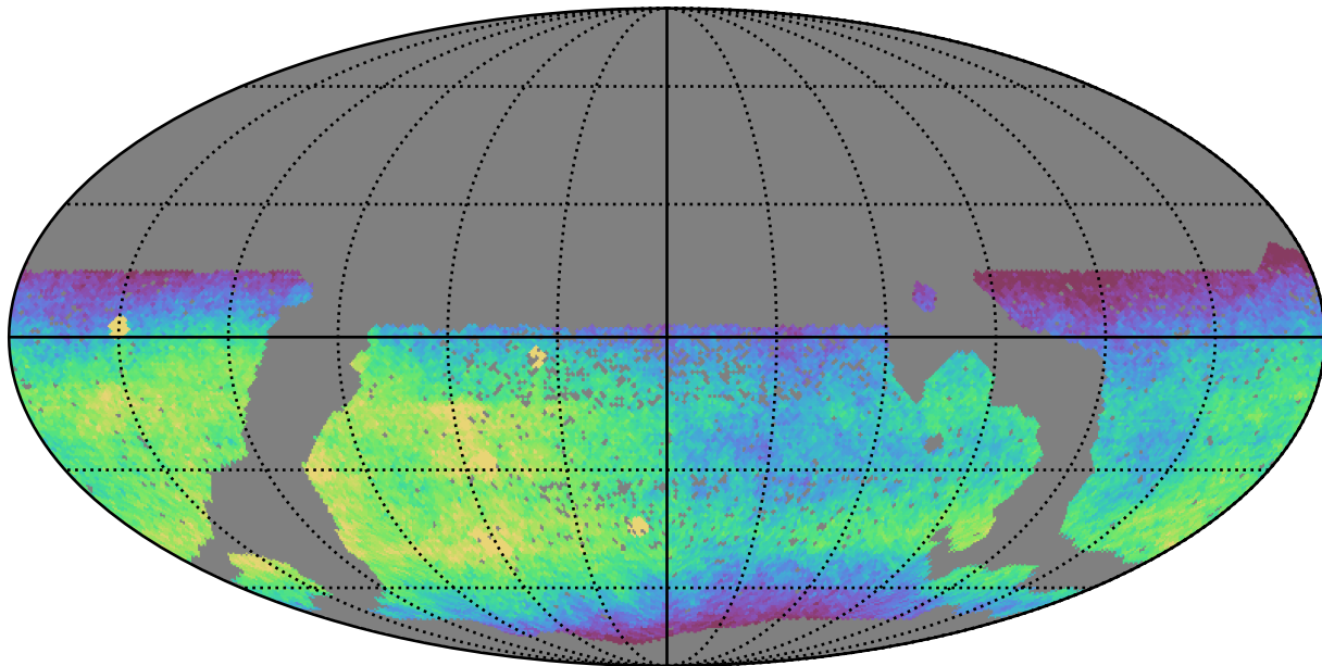
scp_reweight_v3.3_10yrs WFD r band: CoaddM5
