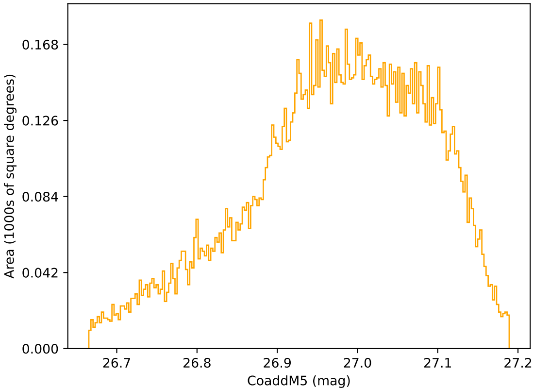
scp_reweight_v3.3_10yrs WFD r band: CoaddM5
