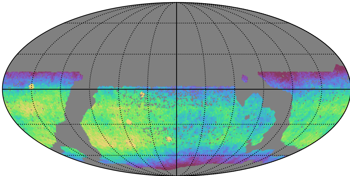
scp_reweight_v3.3_10yrs WFD i band: CoaddM5
