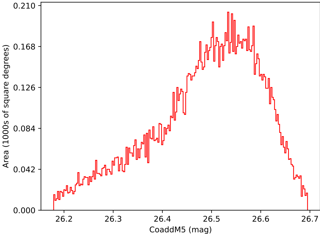
scp_reweight_v3.3_10yrs WFD i band: CoaddM5
