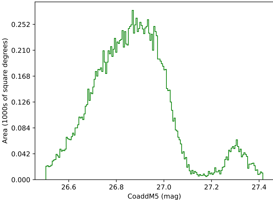
scp_reweight_v3.3_10yrs WFD g band: CoaddM5
