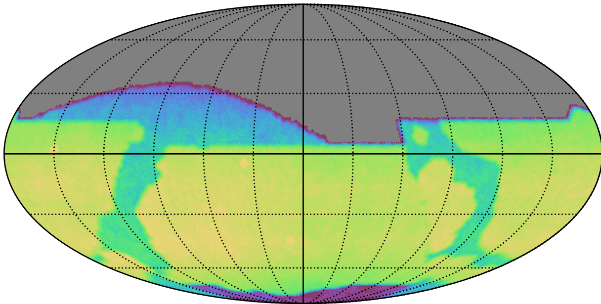
scp_reweight_v3.3_10yrs All sky z band: CoaddM5
