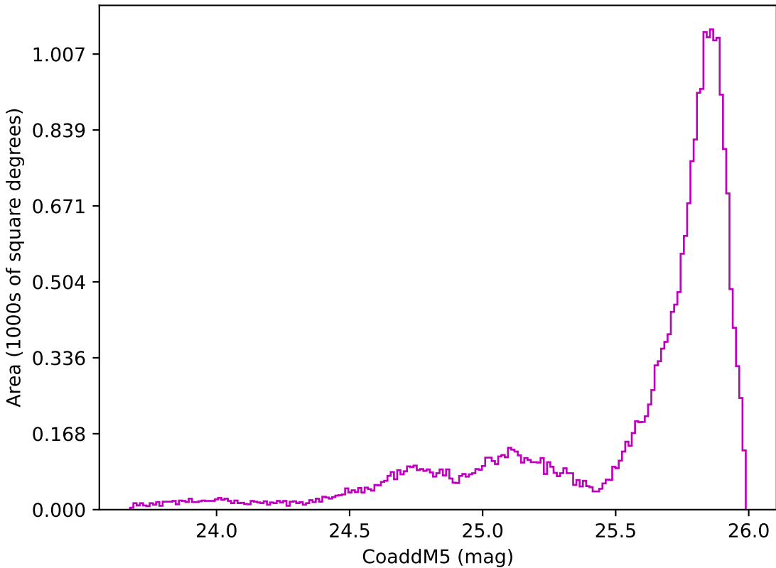
scp_reweight_v3.3_10yrs All sky z band: CoaddM5
