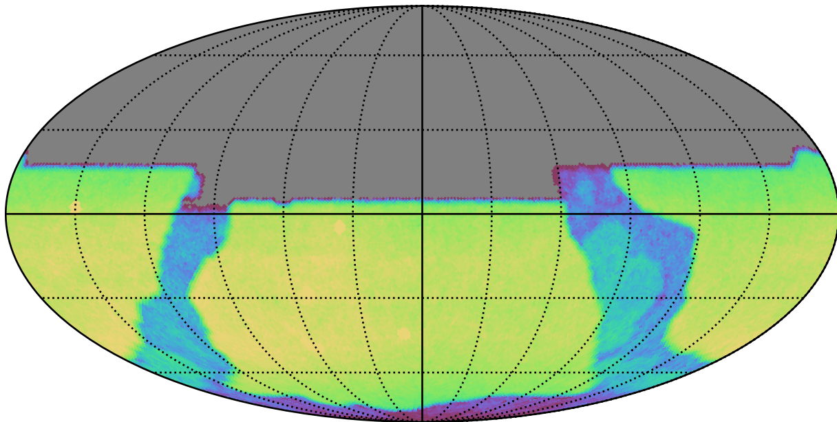
scp_reweight_v3.3_10yrs All sky y band: CoaddM5
