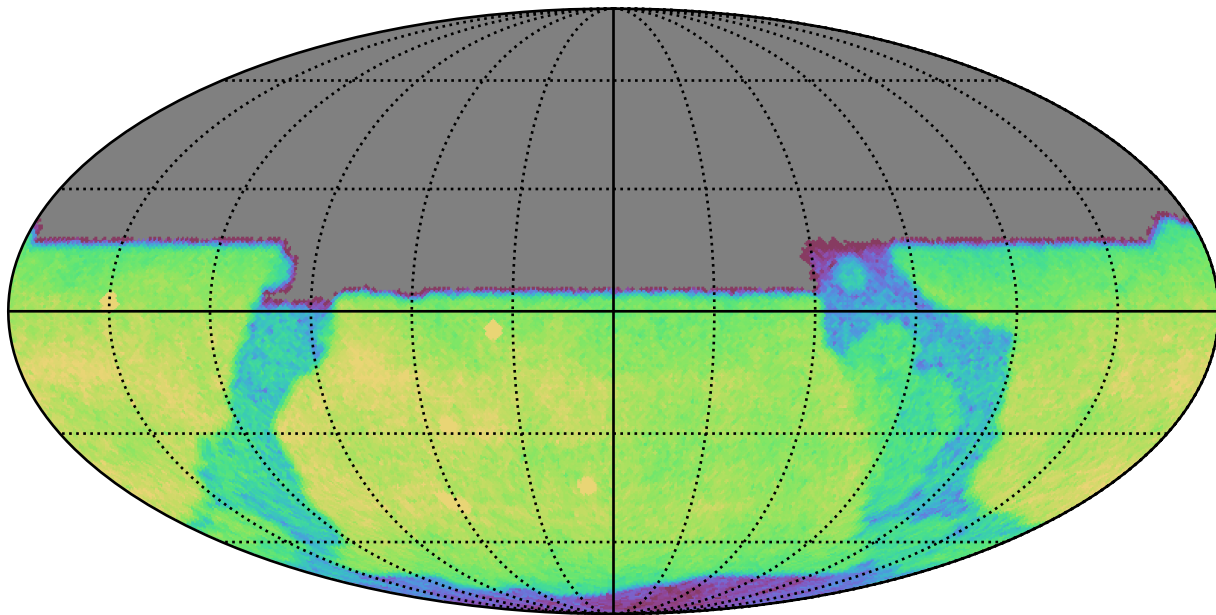
scp_reweight_v3.3_10yrs All sky u band: CoaddM5
