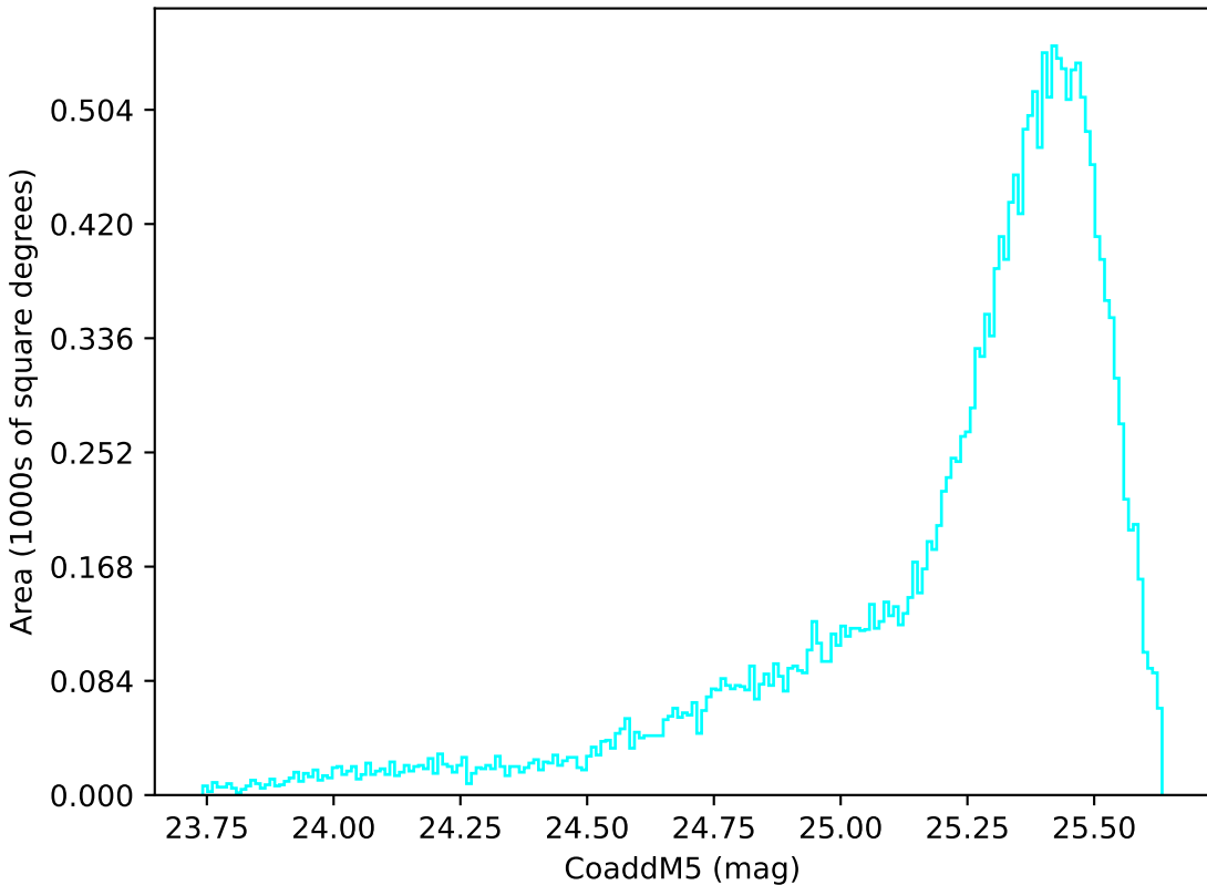
scp_reweight_v3.3_10yrs All sky u band: CoaddM5
