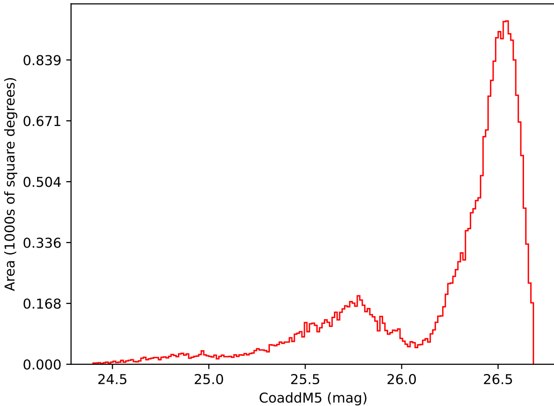
scp_reweight_v3.3_10yrs All sky i band: CoaddM5
