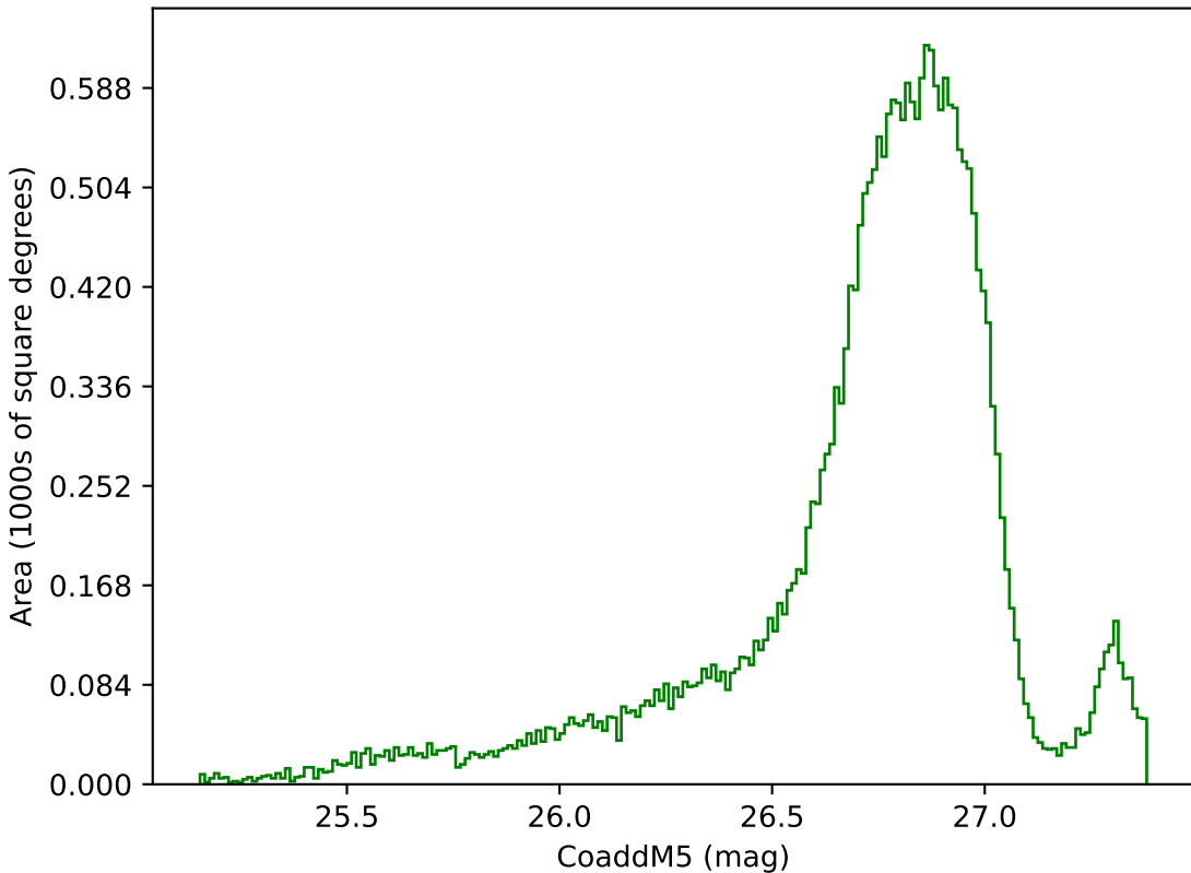
scp_reweight_v3.3_10yrs All sky g band: CoaddM5
