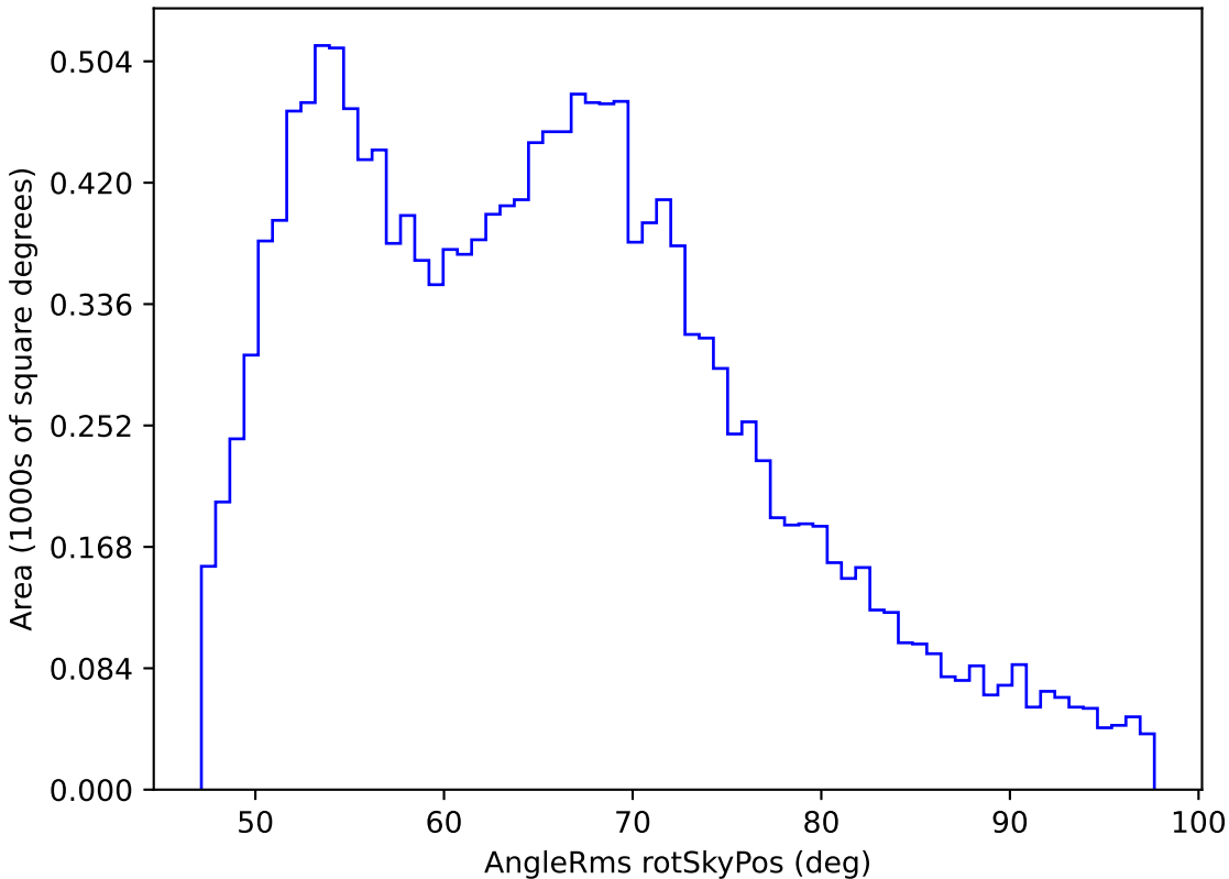
scp_reweight_v3.3_10yrs WFD y band: AngleRms rotSkyPos
