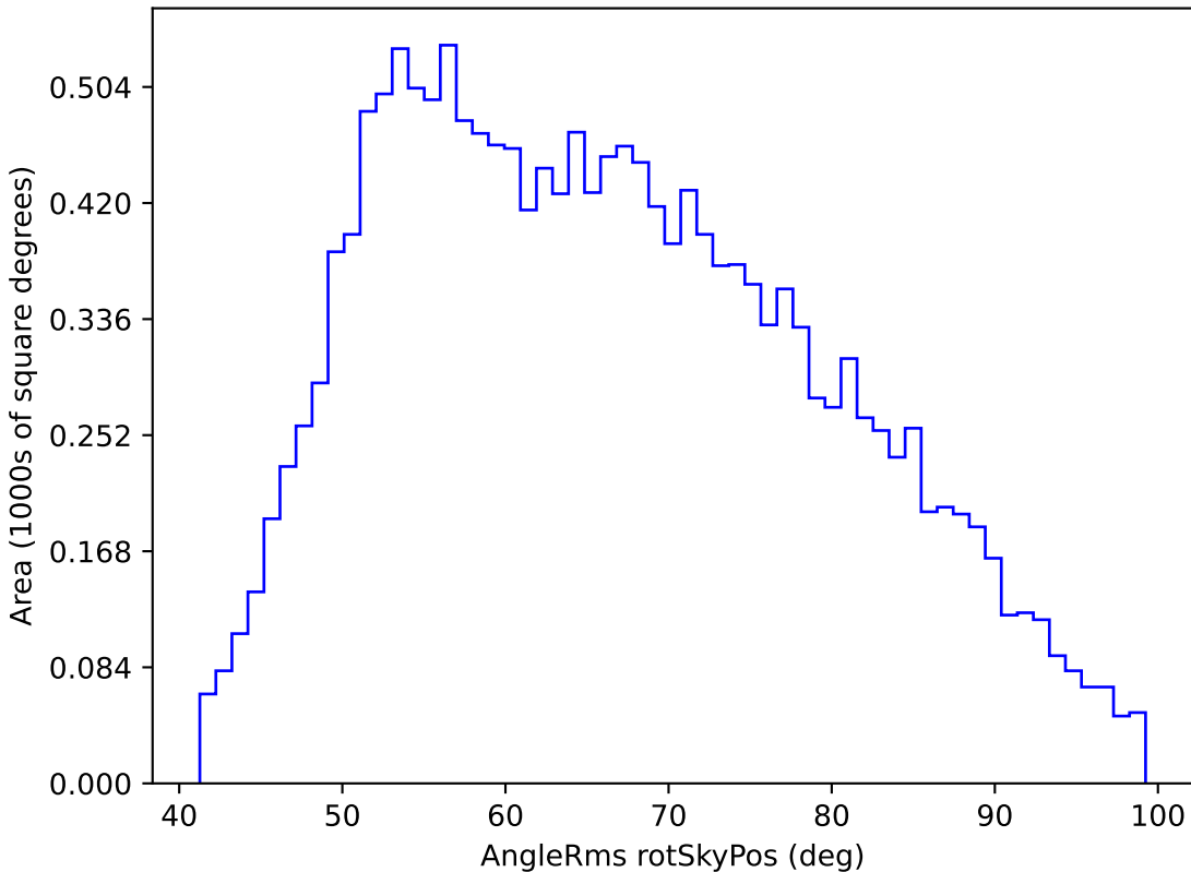
scp_reweight_v3.3_10yrs WFD u band: AngleRms rotSkyPos
