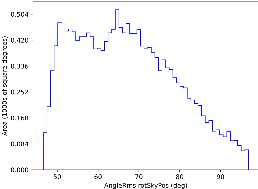
scp_reweight_v3.3_10yrs WFD i band: AngleRms rotSkyPos
