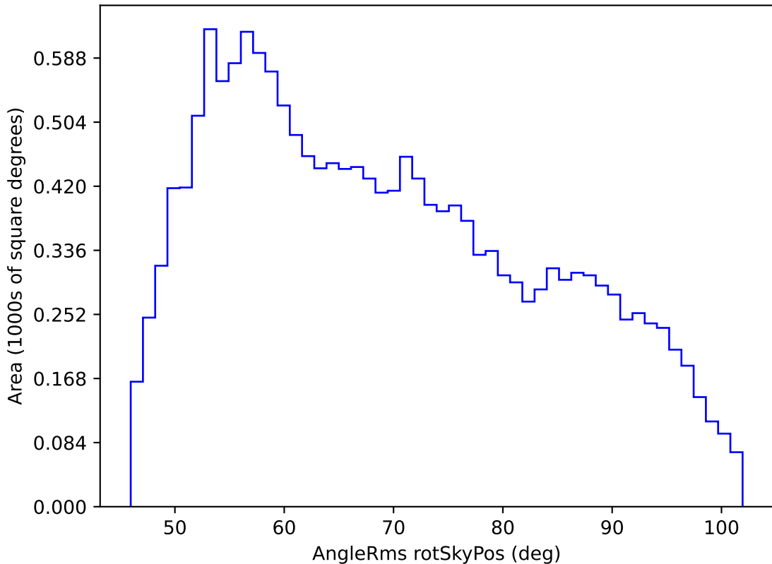
scp_reweight_v3.3_10yrs WFD g band: AngleRms rotSkyPos
